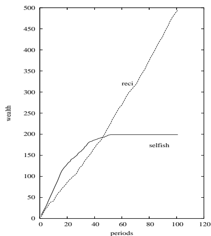
Figure 3: Performance of reciprocal and selfish agents after removing the zero cost identity problem.
