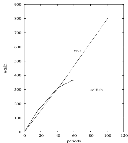
Figure 4: Performance of reciprocal and selfish agents using reputation information from other agents.
